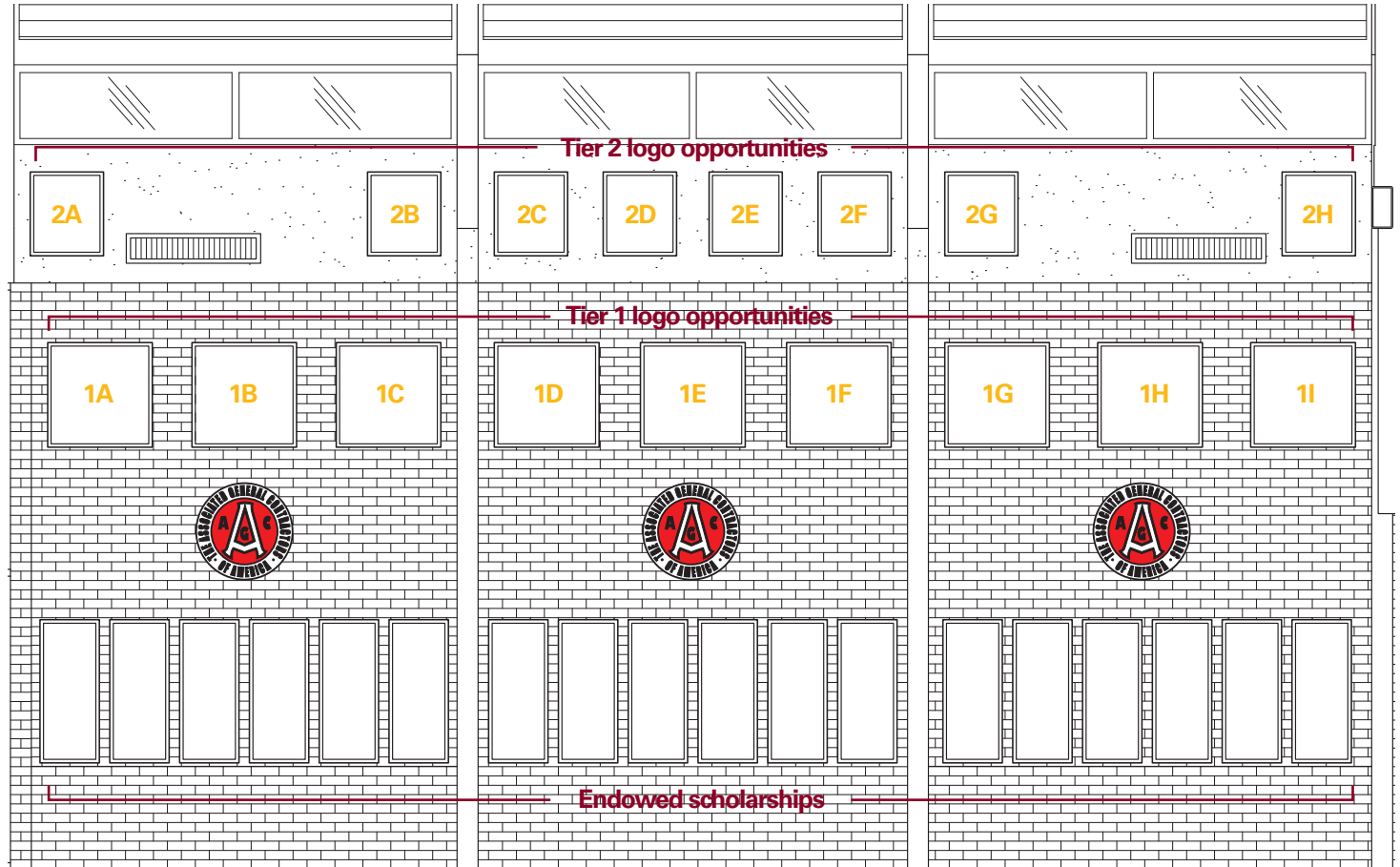
South wall elevation (interior)
